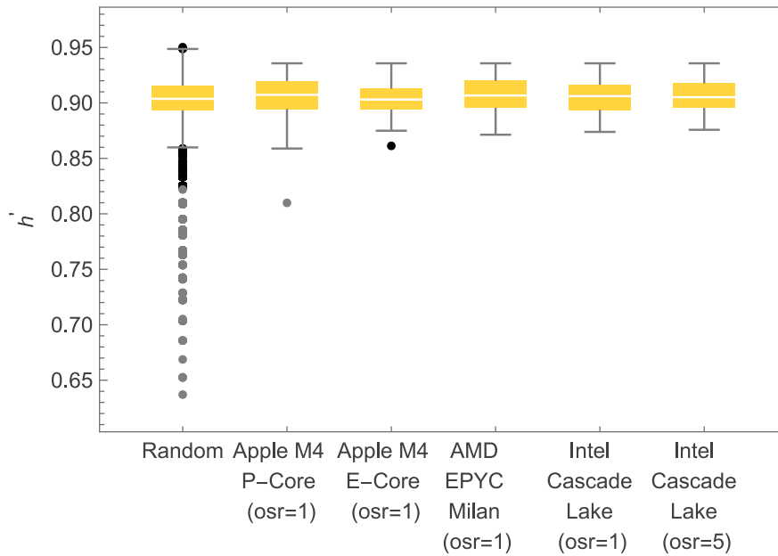
Figure 13. Random Data Assessments ( n = 10^6 ) Compared to LFSR Conditioned Data Assessments (Each n = 100 )
